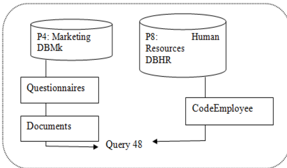
Fig. 4. A second query between DBMk and DBHR
